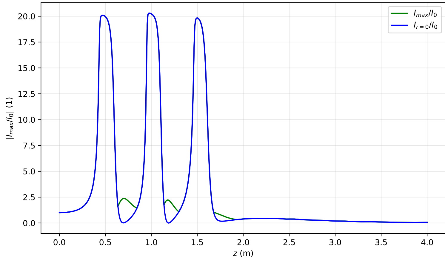
I_{max}(x = 0, y = 0, z)/I_0 , \text{Pin}=5.5\text{Pcr} , artificial time
